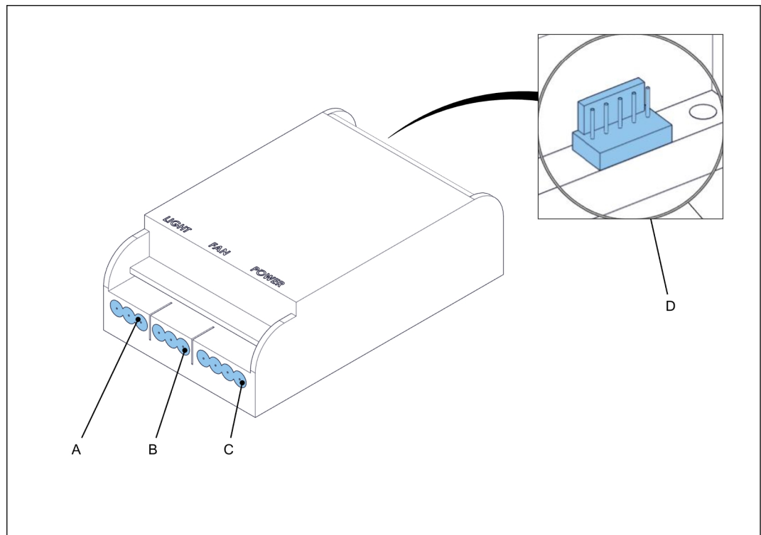
Figure 5. Fan/light module
