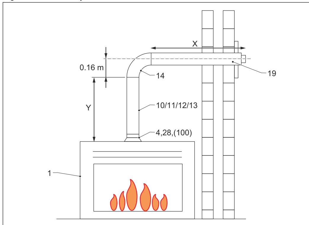
Concentric flue connection on appliance \text{\O}100\text{-}\text{\O}150 mm or \text{\O}130\text{-}\text{\O}200 mm
