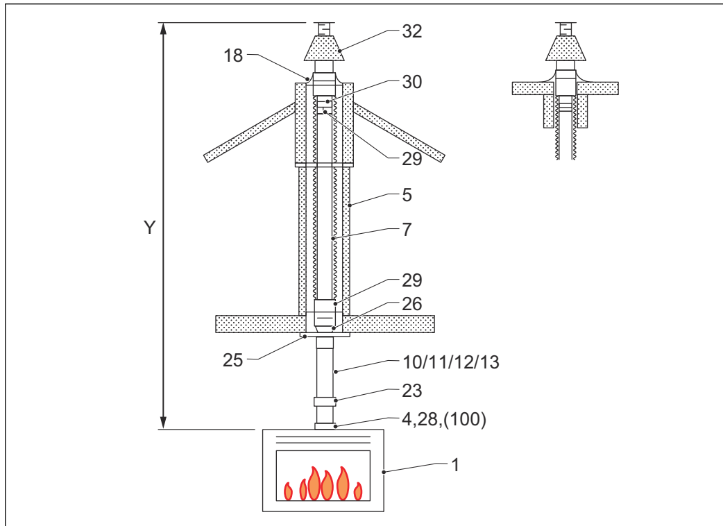
Concentric flue connection on appliance \varnothing 100\text{-}\varnothing 150 mm or \varnothing 130\text{-}\varnothing 200 mm
