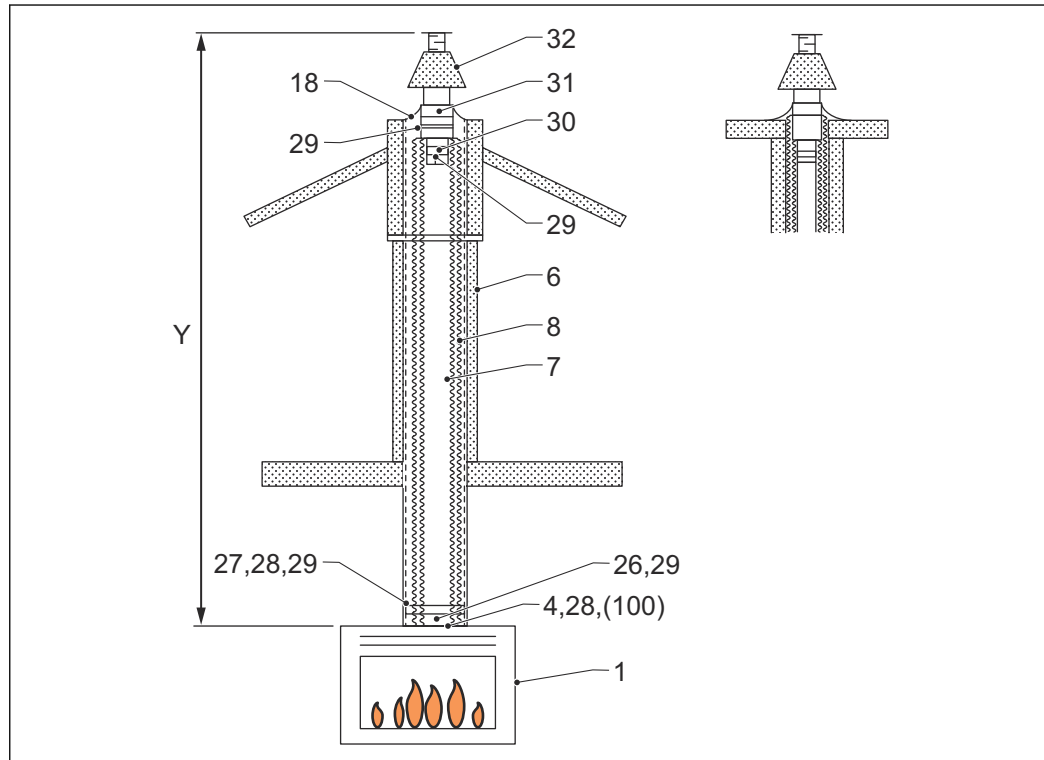
Concentric flue connection on appliance \text{Ø}100\text{-}\text{Ø}150 mm or \text{Ø}130\text{-}\text{Ø}200 mm
