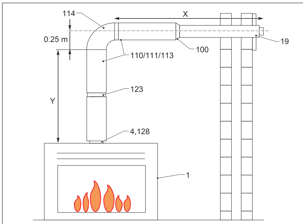
Concentric flue connection on appliance \varnothing 130\text{-}\varnothing 200 mm
