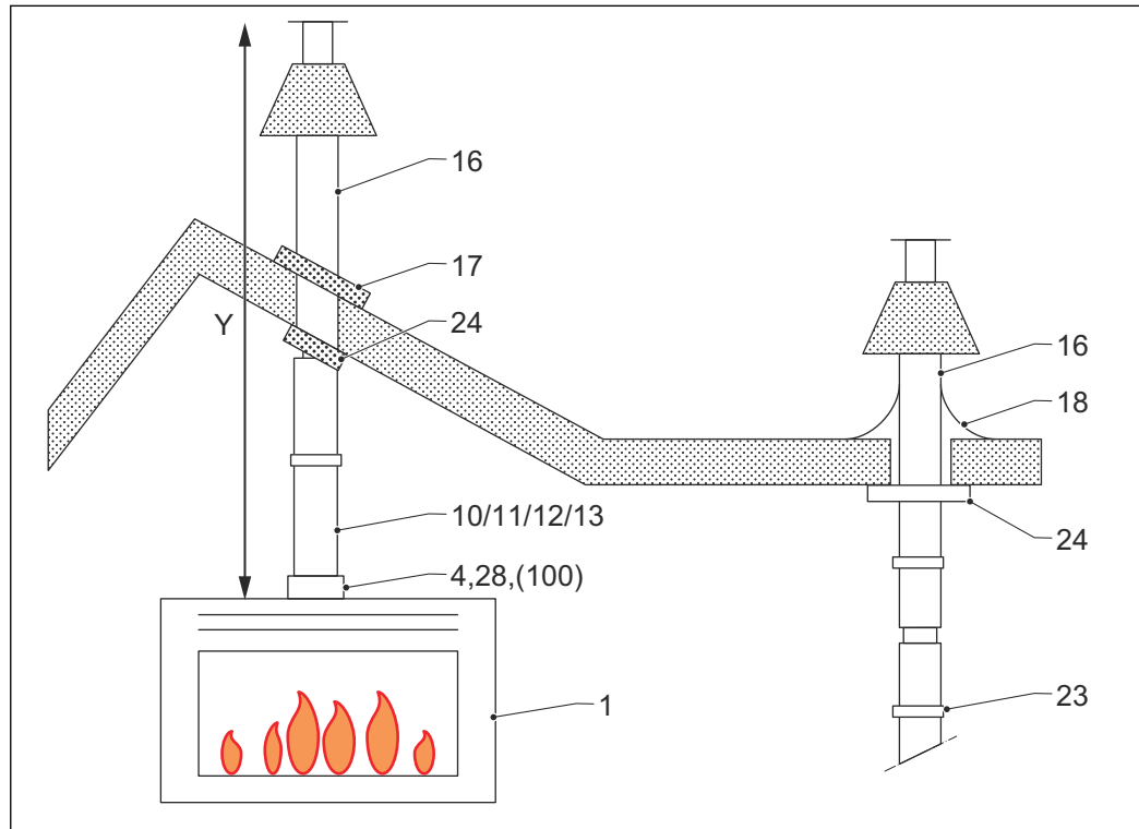
Concentric flue connection on appliance \text{Ø}100\text{-}\text{Ø}150\text{ mm} or \text{Ø}130\text{-}\text{Ø}200\text{ mm}
