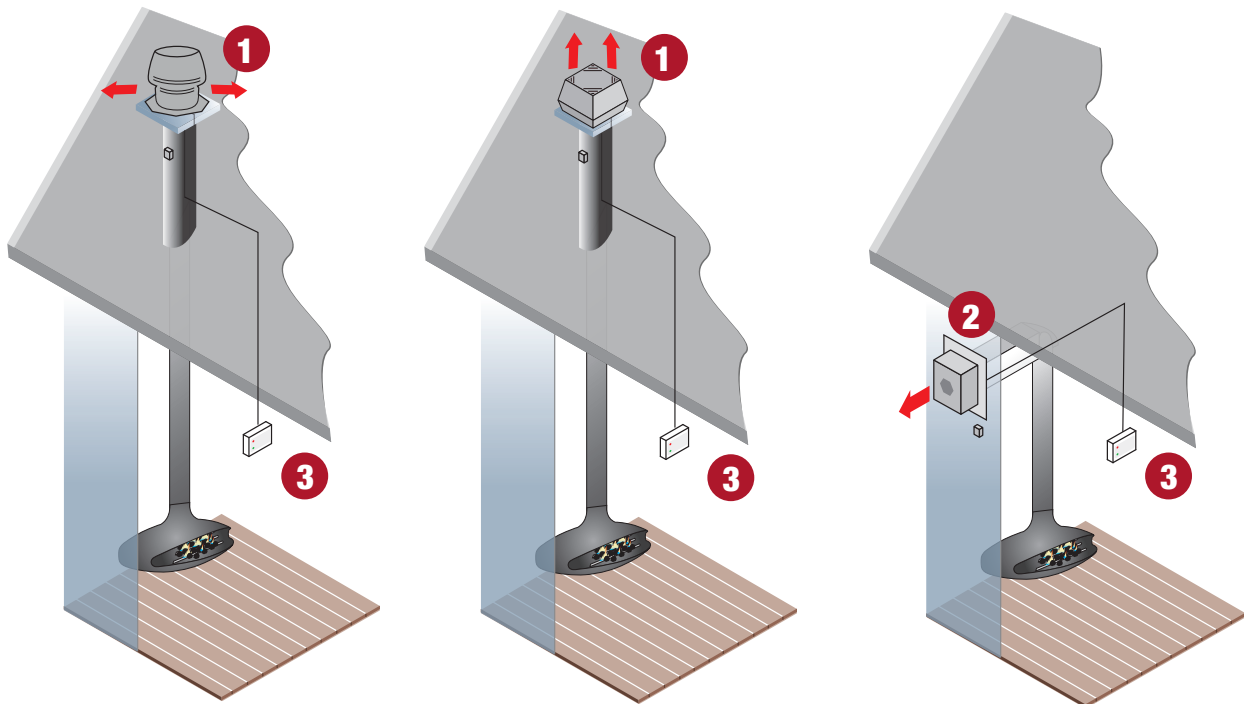
Chimney fan system with horizontal extraction via a steel chimney
